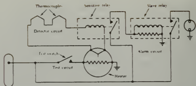
FIGURE 9-2. Thermocouple fire warning circuit.
